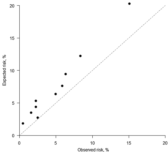
Figure 6 Calibration plot, applied to the testing cohort. Expected risk (from the best model from figure 3 : see box 1 ) versus the observed risk (relative frequency of cardiovascular disease events) in the testing cohort of non-Glaswegian women. Results are shown for the (approximately) equal number of women in each of the tenths of expected risk.
